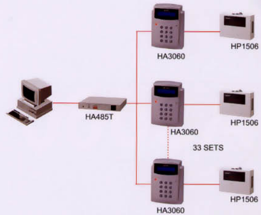
Network configuration upto 32 sets with HA485 connected
