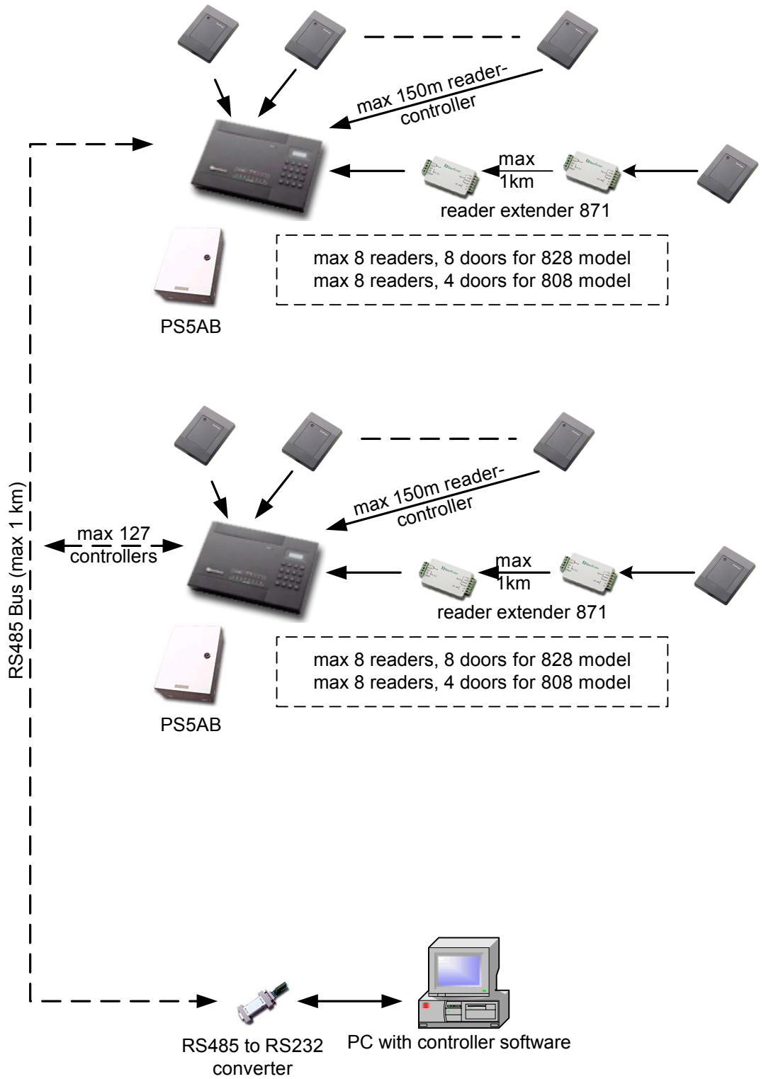
Fig 1. RS485 Network Connection Diagram for Everfocus Access Control System (option 1)
